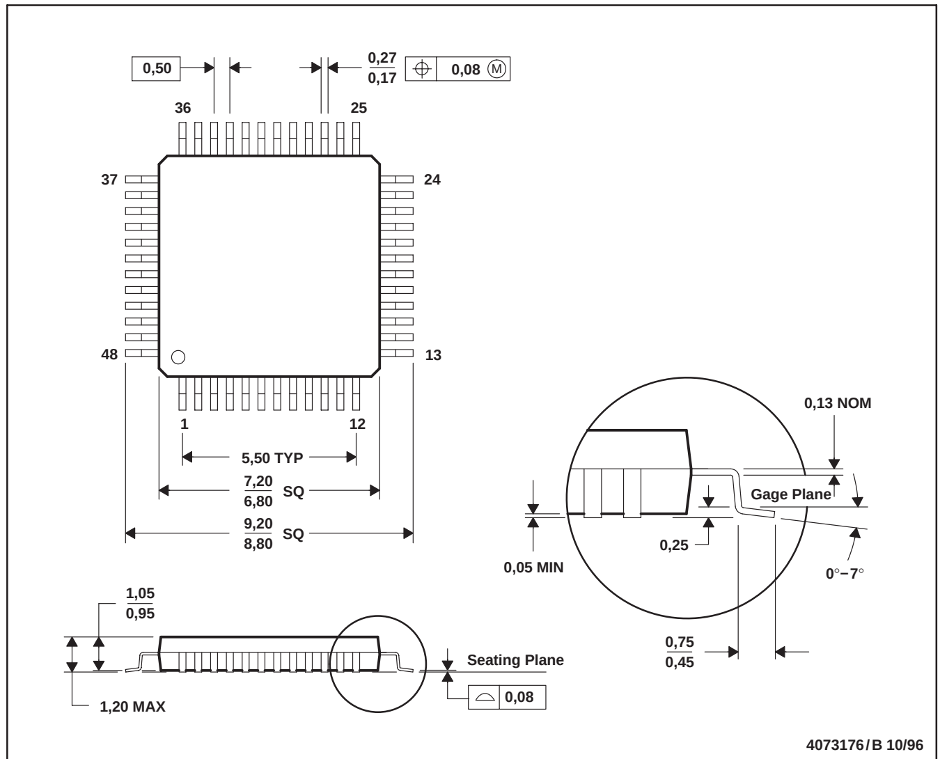
PFB (S-PQFP-G48)
