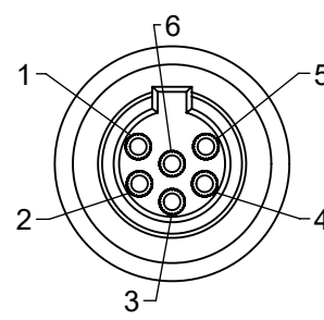
TB6MS 6 PIN
