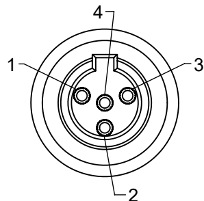
TB4MS 4 PIN
