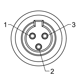
TB3MS 3 PIN
