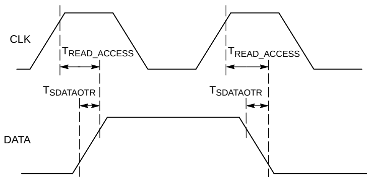
Figure 10. MIPI-RFFE Signal Timing during Master Reads from PTIC Control IC
