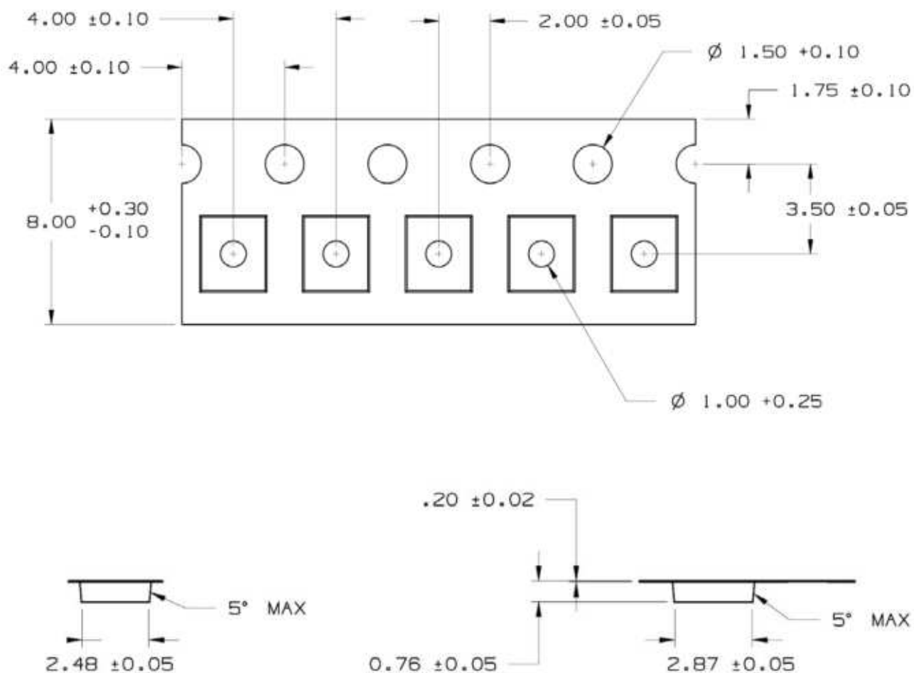
Figure 18. WLCSP Carrier Tape Drawings
