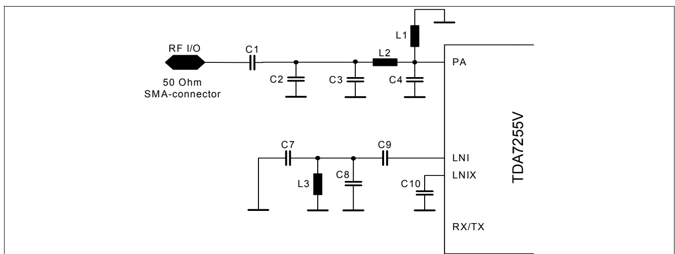
Figure 25 TX_Mode_Simplified
