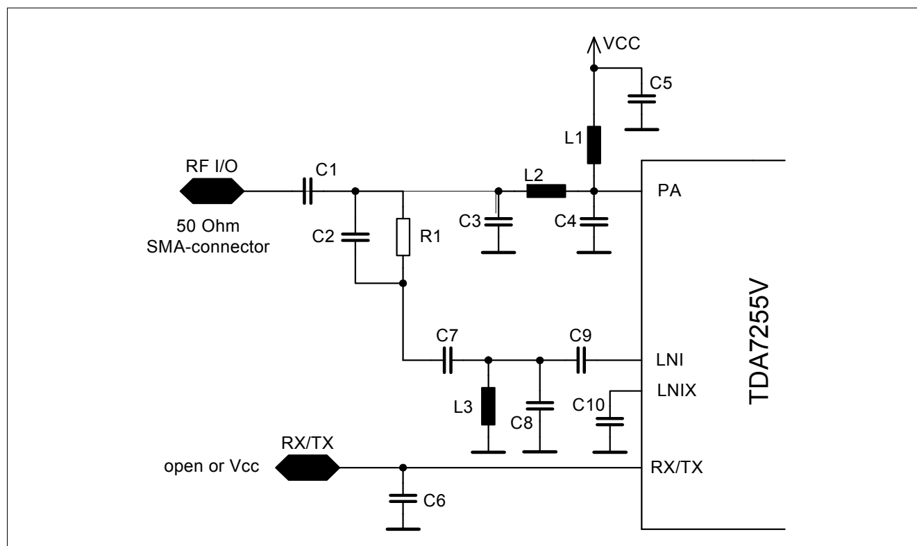
Figure 22 RX-Mode
