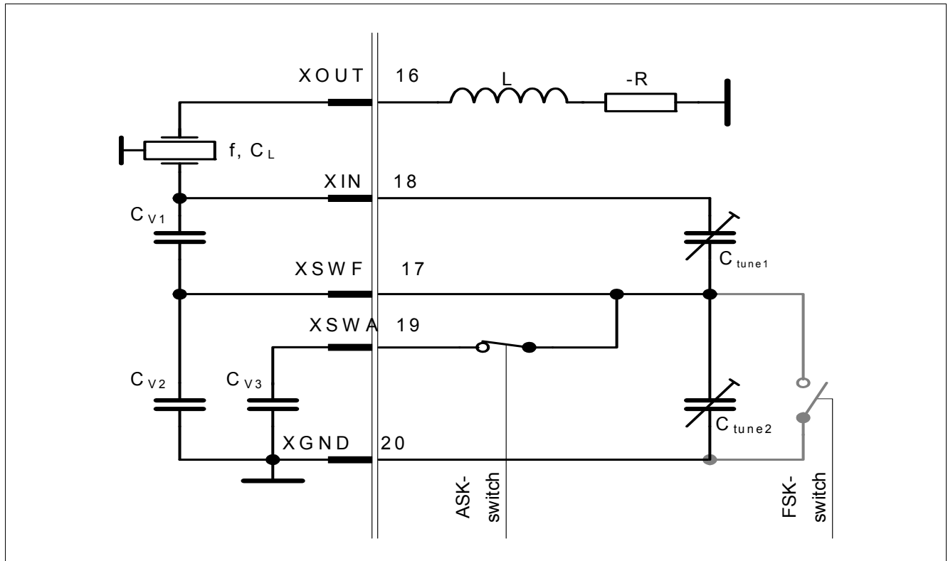
Figure 36 FSK Receive
