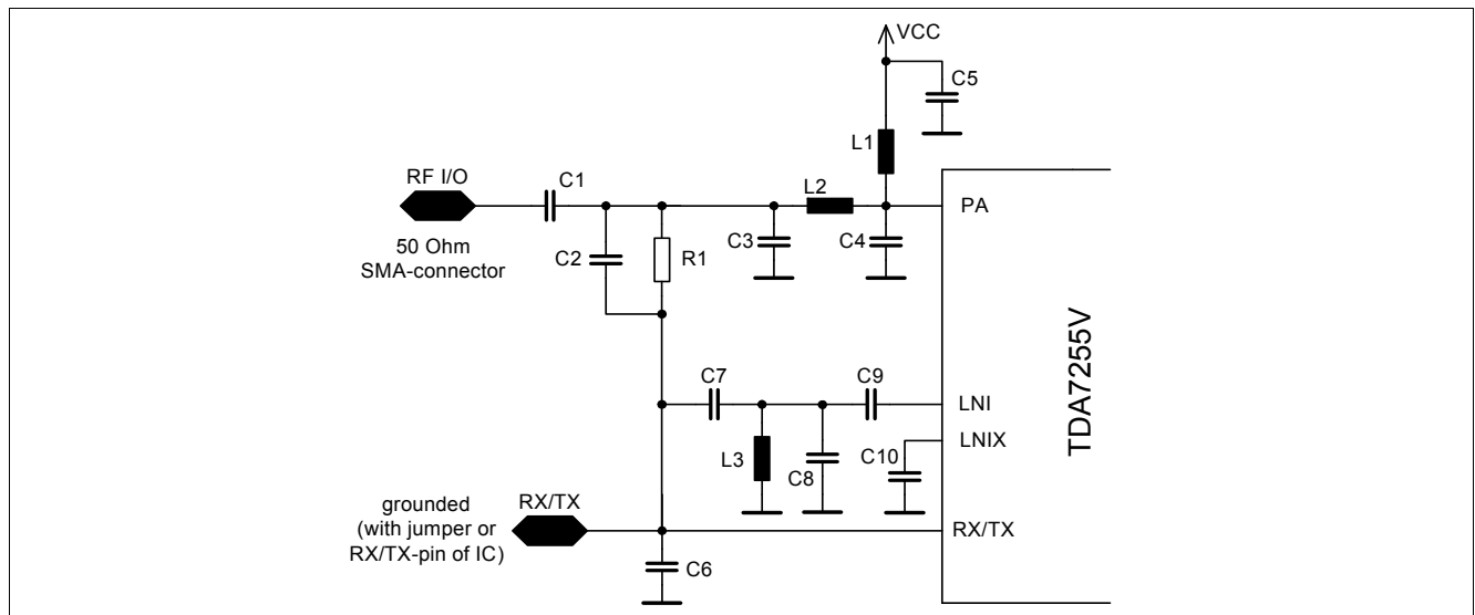
Figure 24 TX_Mode
