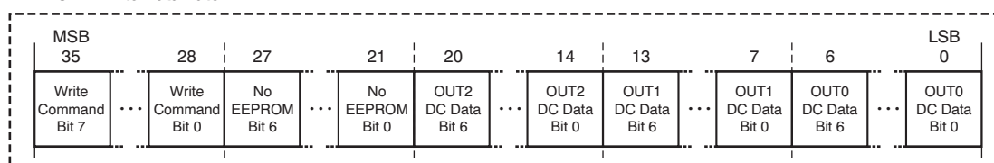
Figure 33. EEPROM2 Write Data Latch Bit Assignment
