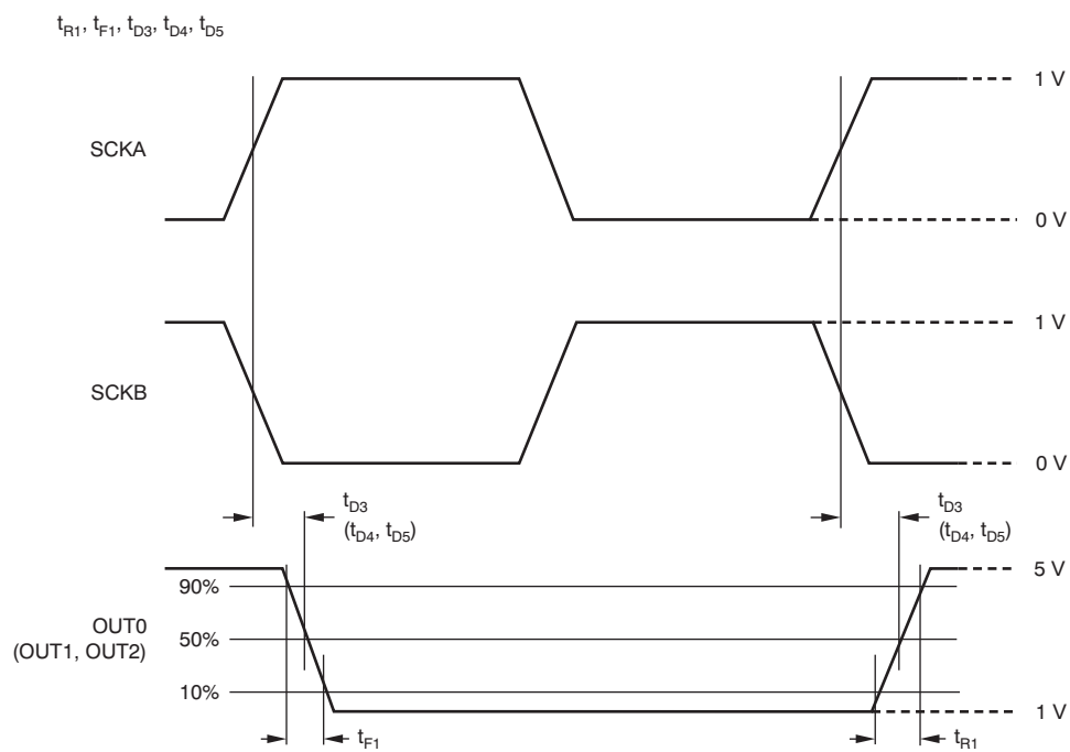
Figure 12. Output Timing
