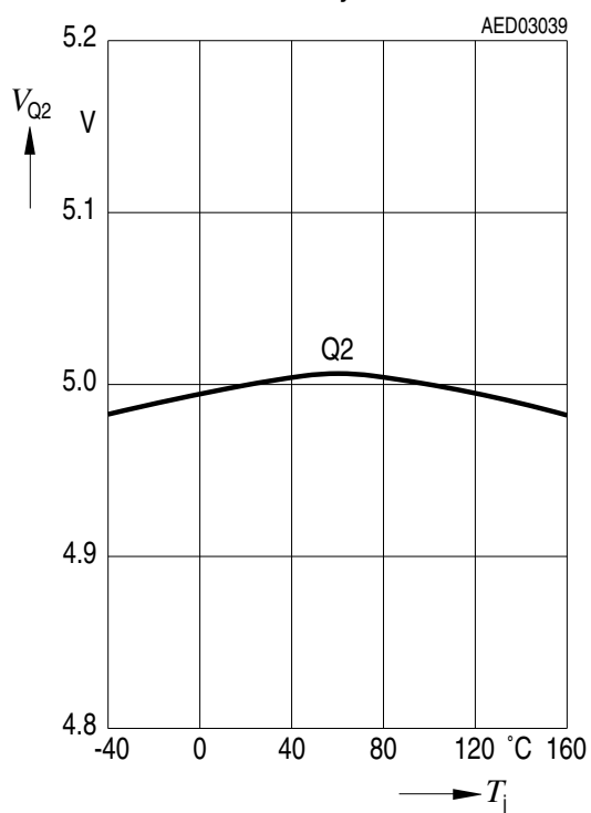
Output Voltage V_{Q2} versus Temperature T_j
