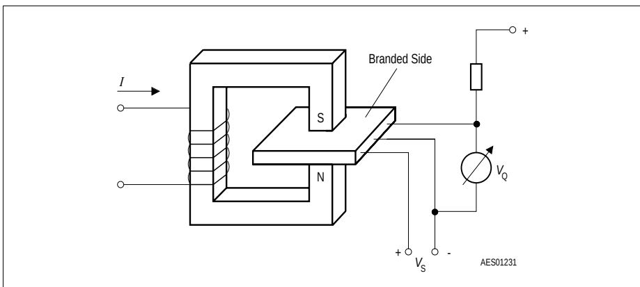
Figure 3 Sensor/Magnetic-Field Configuration
