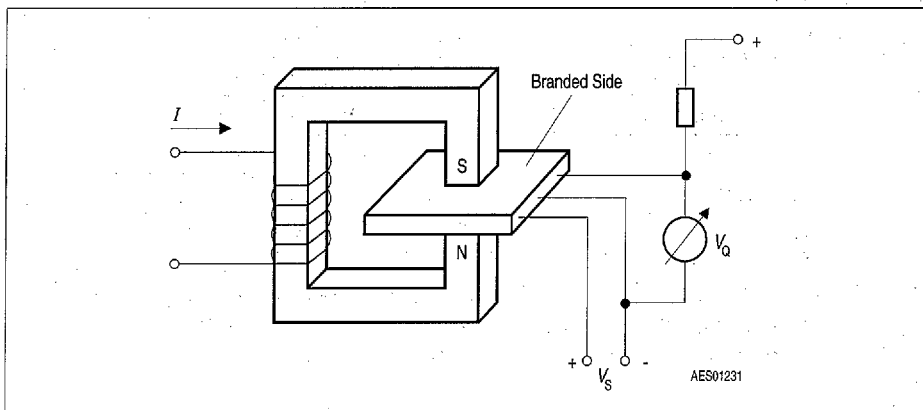
Figure 5 Sensor/Magnetic-Field Configuration
