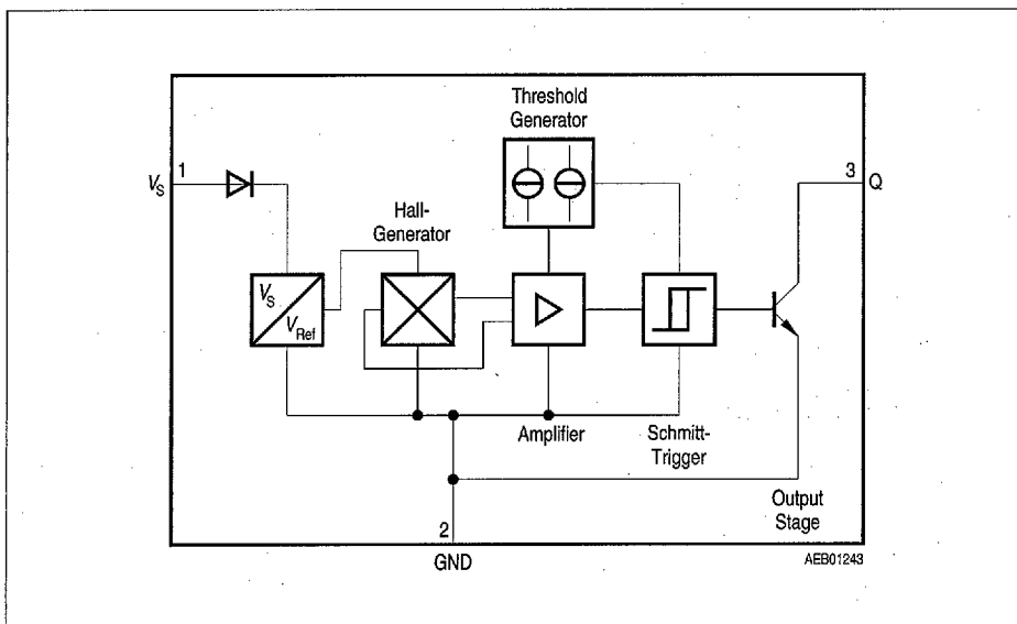
Figure 2 Block Diagram
