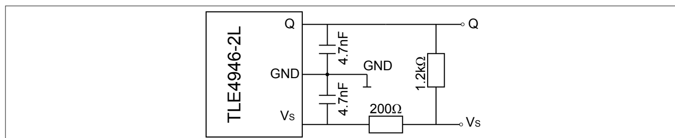
Figure 5 Application circuit
