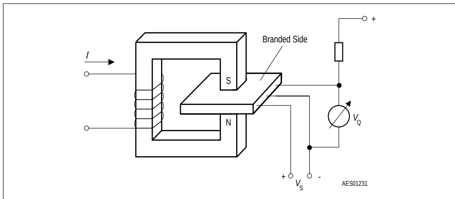
Figure 5 Sensor/Magnetic-Field Configuration
