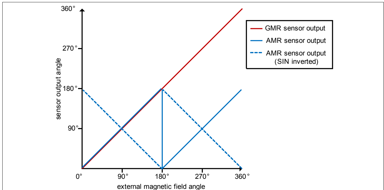
Figure 8 Dual die angle output
