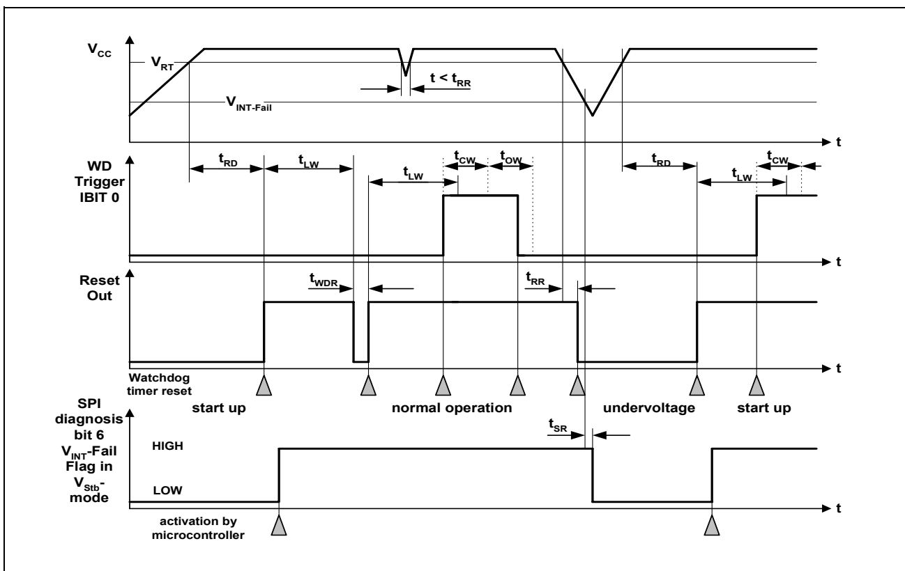
Figure 13: Reset Timing Diagram
