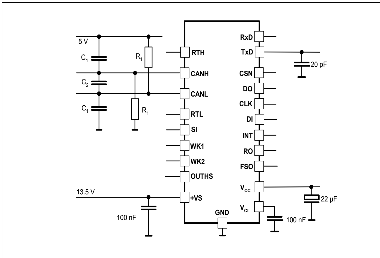
Figure 14: Test Circuit
