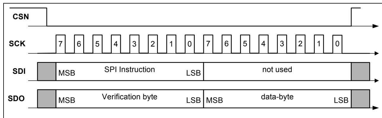
Figure 8 SPI communication
