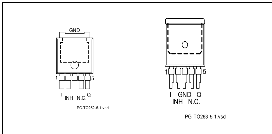
Figure 2 Pin Configuration P-T0252-5 (D-PAK), P-T0263-5 (D 2 -PAK)(top view)
