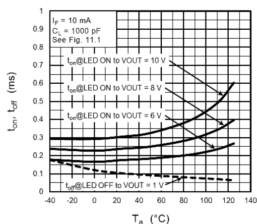
Fig. 12.12 t_{on}, t_{off} - T_a
