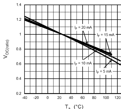
Fig. 12.8 V_{OC(ratio)} - T_a
