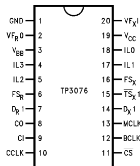
Figure 1. See Package PDIP (NHF)
