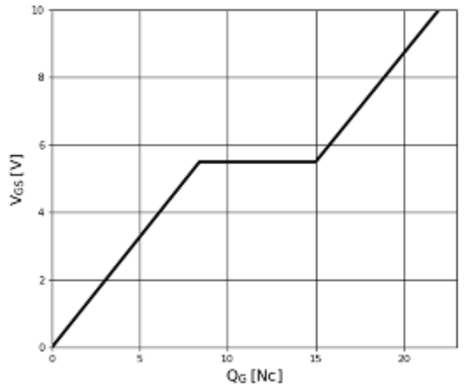
Figure 8. Typical Gate Charge
