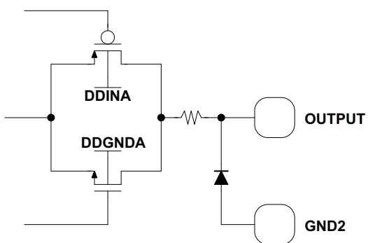
Figure 62. ERR
