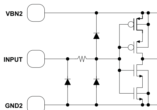
Figure 51. REG_EN
