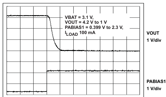
BUCK BOOST/OUTPUT VOLTAGE SETTLING TIME
