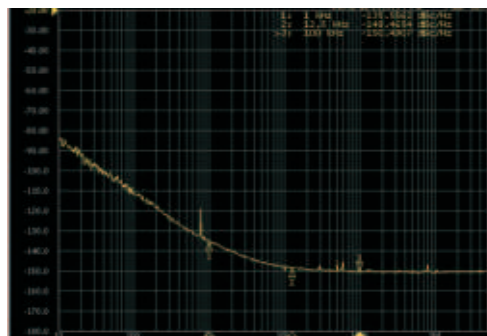
SYSCLK_IN (VTCXO OUTPUT) INPUT PHASE NOISE
