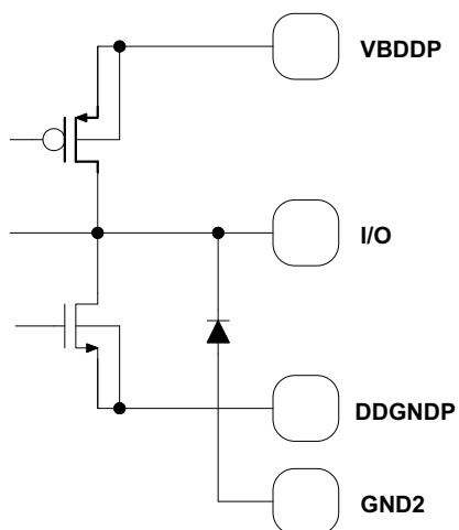
Figure 64. L1
