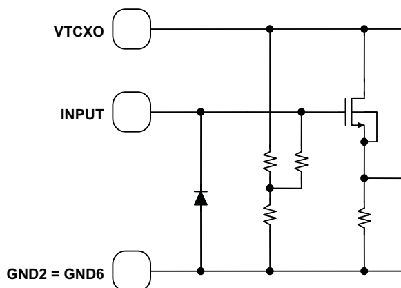
Figure 59. SYSCLK_IN
