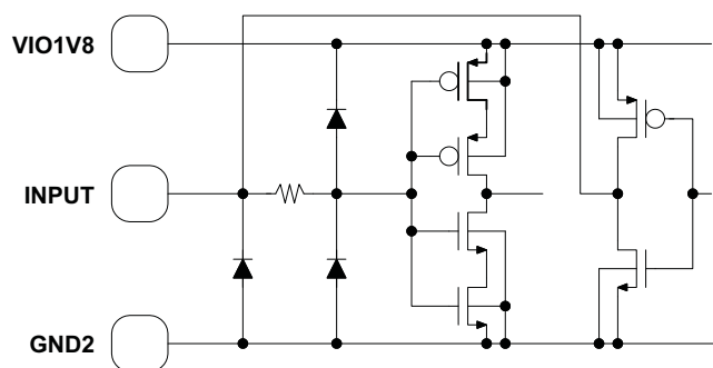
Figure 52. CDATA
