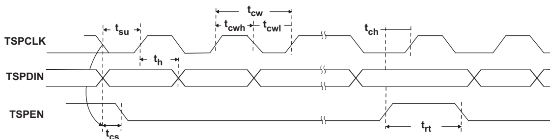
Figure 90. TSP Timing
