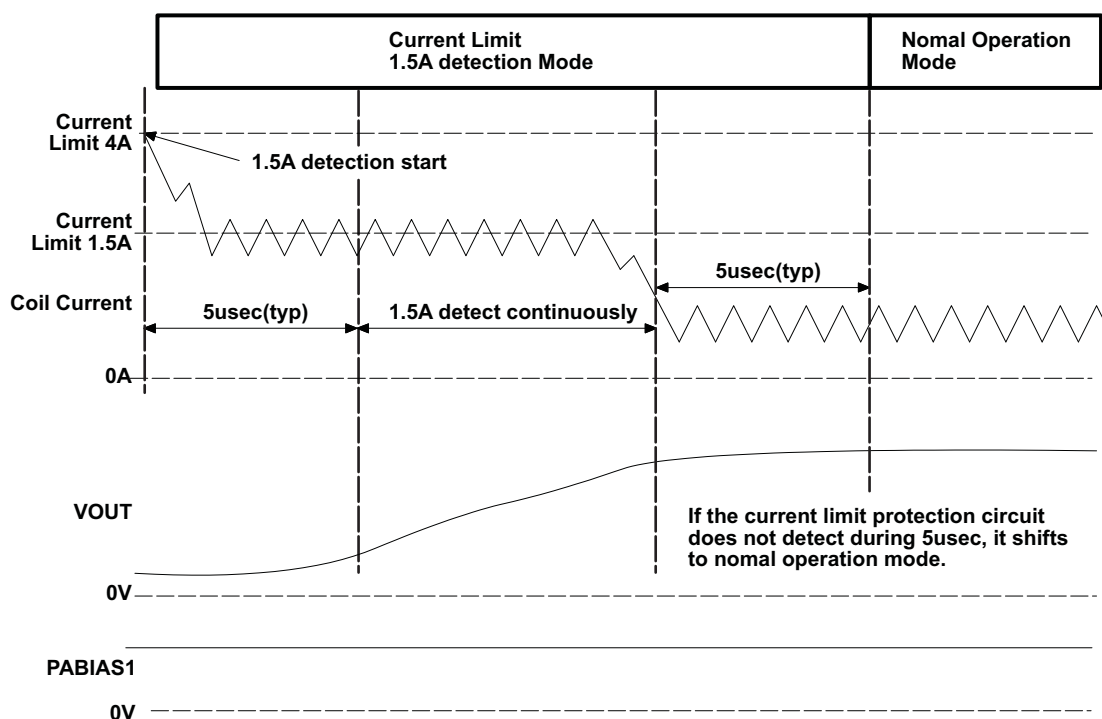
(c) 1.5 A Detection
