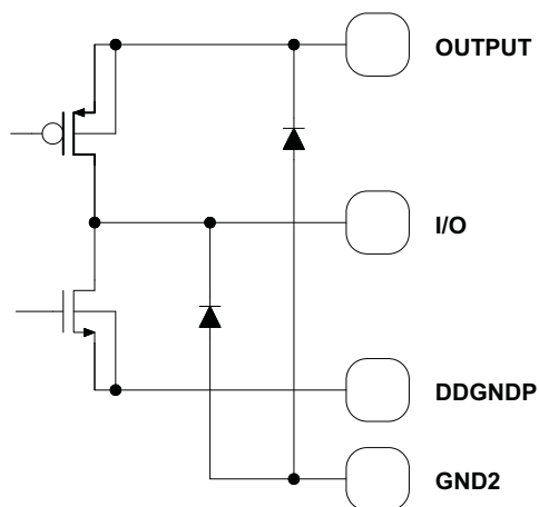
Figure 65. VOUT, L2
