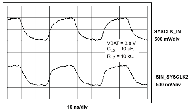
CLOCK DISTRIBUTION/SIN_SYSCLOCK2 INPUT vs OUTPUT (–1 dB TYP)
