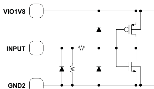
Figure 49. TXONFST, TXON, TBNDSSEL2, TBNDSSEL1
