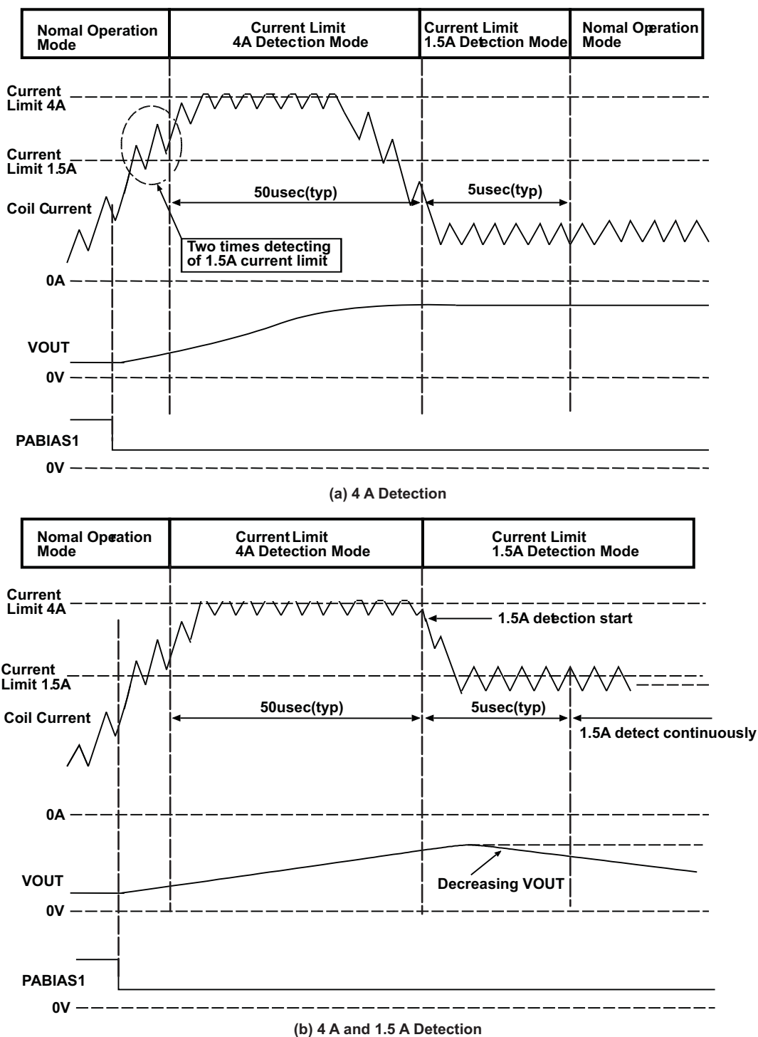
Figure 73. Current Limit Protection - View (a) and (b)
