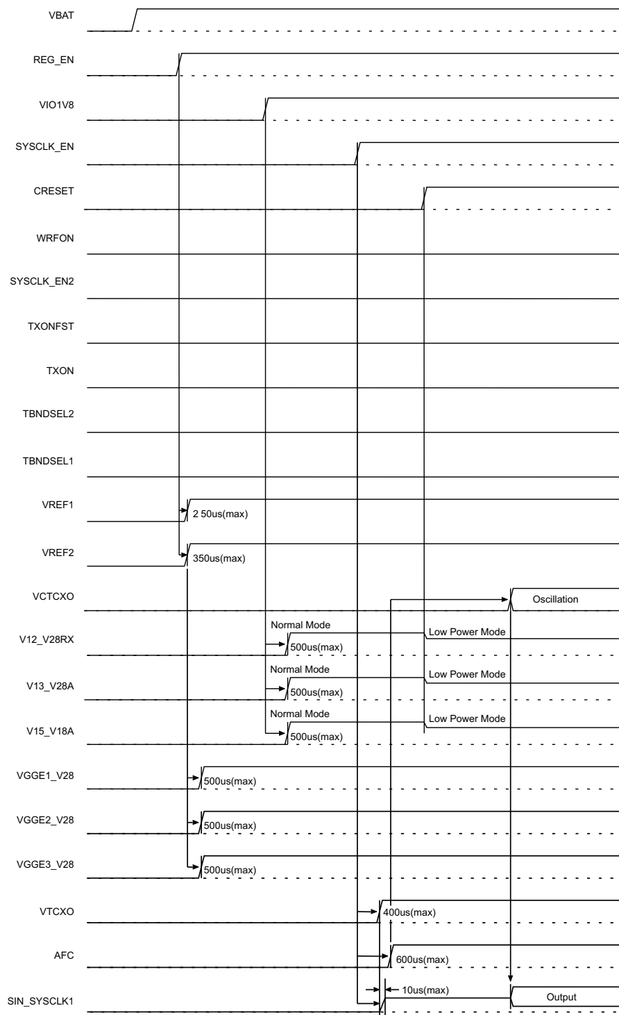
Figure 84. Power-Up Sequence
