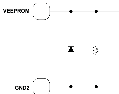
Figure 69. VEEPROM
