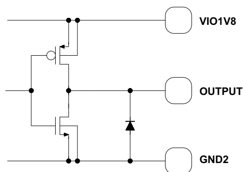
Figure 53. EXT_DC_DC_ON_OFF
