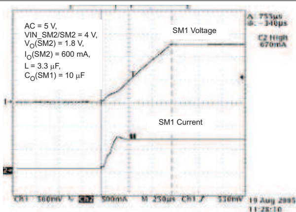
Figure 54. Transient - SM1 Start-Up
