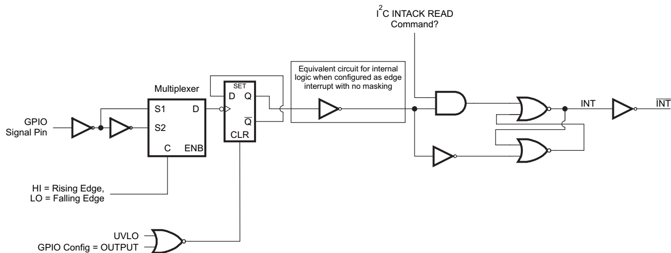
Figure 47. GPIO 1 or GPIO2 Configured as an Interrupt Request Input
