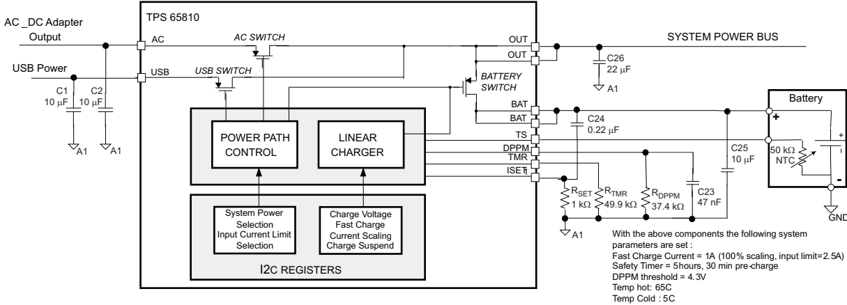
Figure 58. Required External Components, Recommended Values, External Connections
