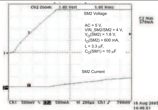
Figure 55. Transient - SM2 Start-Up
