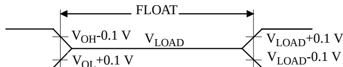
Figure 20. Float Waveforms
