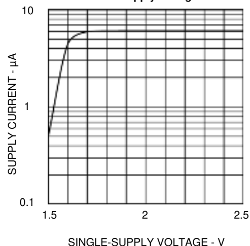
TSM924 Supply Current vs Low Supply Voltages
