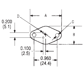
TO-66
