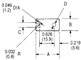
TO-66 (RECTANGLE)
