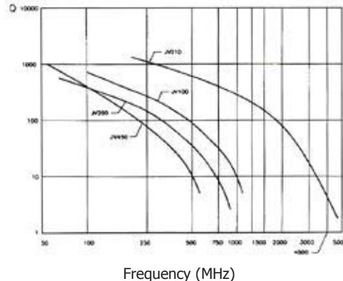
Quality Factor (Q) of “JV” Series Capacitors
