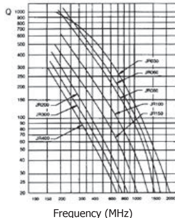
Quality Factor (Q) of “JR” Series Capacitors
