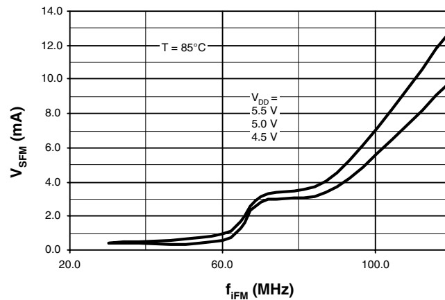
Figure 3. FM Input Sensitivity, T = 85^\circ\text{C}
