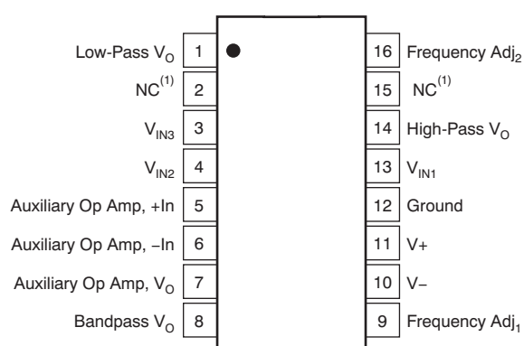
U PACKAGE SOIC-16 (TOP VIEW)
