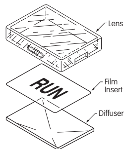
Rectangular Cap
