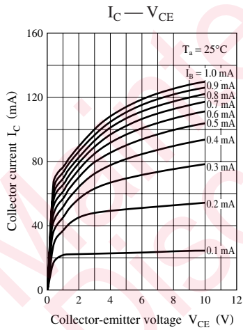
Characteristics charts of UNR521ZG
