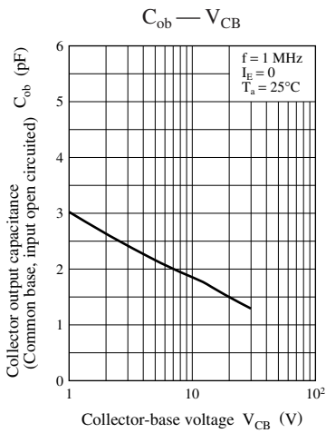
Characteristics charts of UNR521ZG
