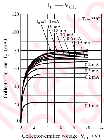
Characteristics charts of UNR5217G
