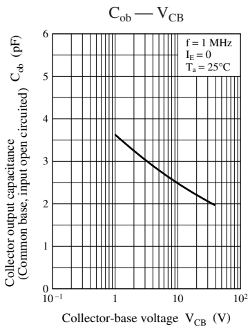
Characteristics charts of UNR521KG
