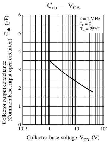
Characteristics charts of UNR5217G
