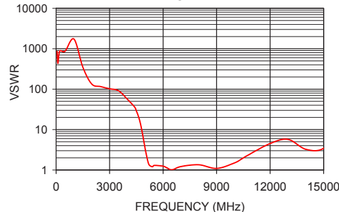
VHF-5050+ VSWR
