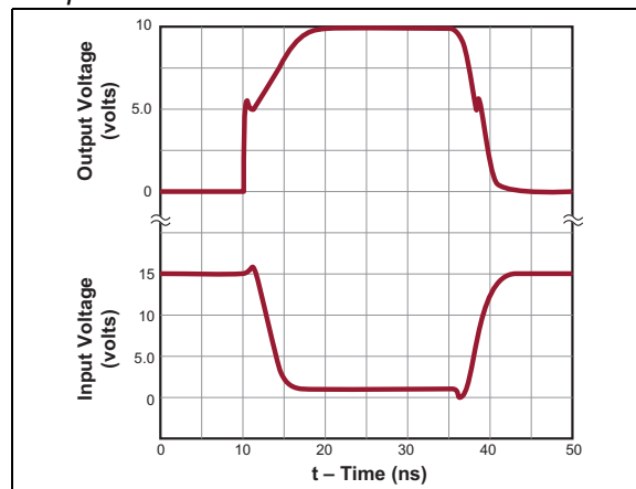
FIGURE 2-6: Switching Waveform.
