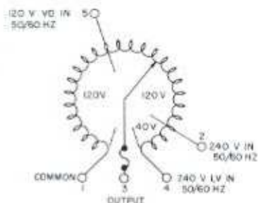
5021 Ganged Unit
