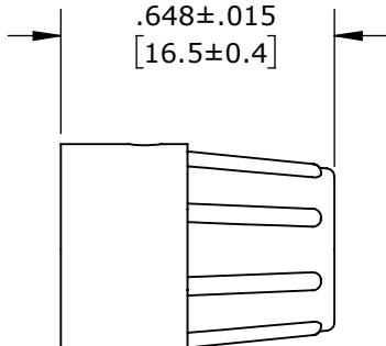
BACKSHELL MAT'L: THERMOPLASTIC, BLACK
