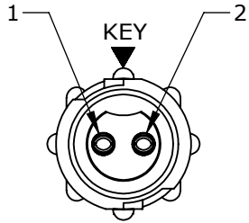
FACE VIEW W18280-2SG-P-3XX
