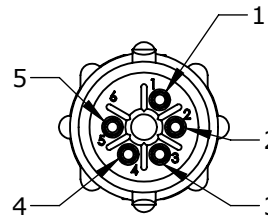
WIRING VIEW W18980-5SG-P-5XX
