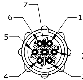
WIRING VIEW W18980-7SG-P-5XX
