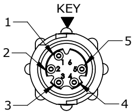
FACE VIEW W18980-5SG-P-5XX 5 POSITION
