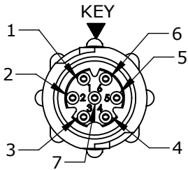
FACE VIEW W18980-7SG-P-5XX 7 POSITION
