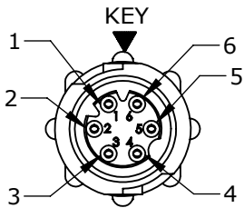
FACE VIEW W18980-6SG-P-5XX 6 POSITION
