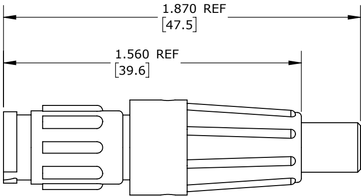
ASSEMBLED VIEW FOR CUSTOMER REF. ONLY
