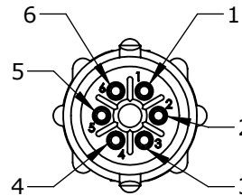
WIRING VIEW W18980-6SG-P-5XX
