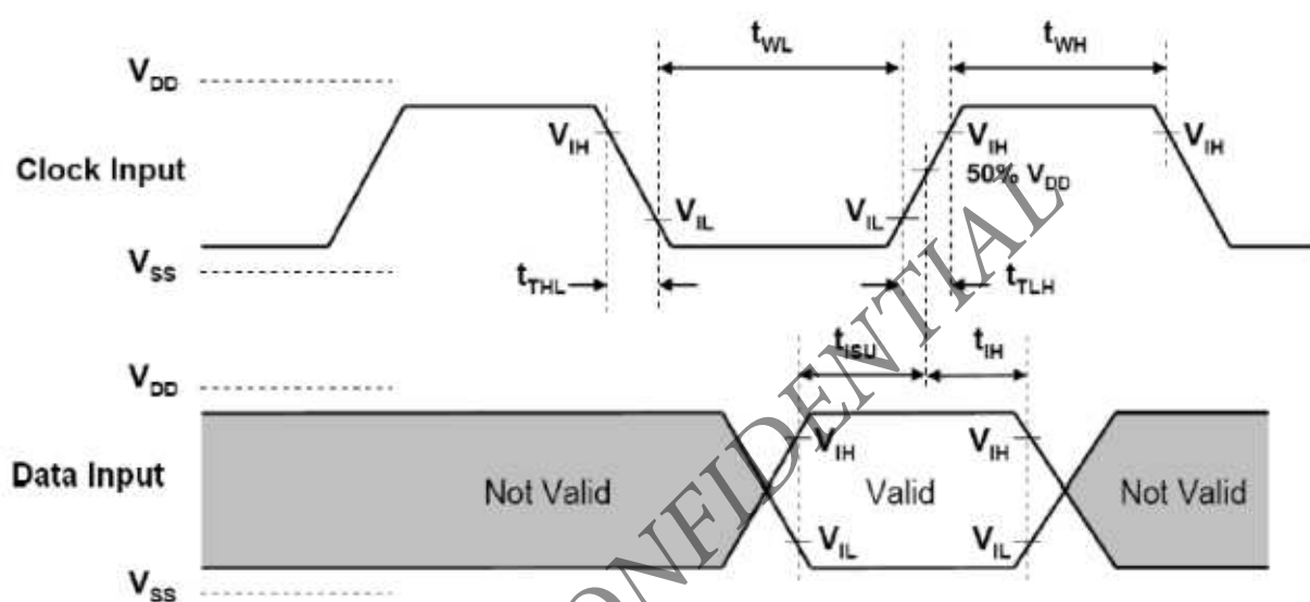
Figure 5-3. SDIO HS input timing
