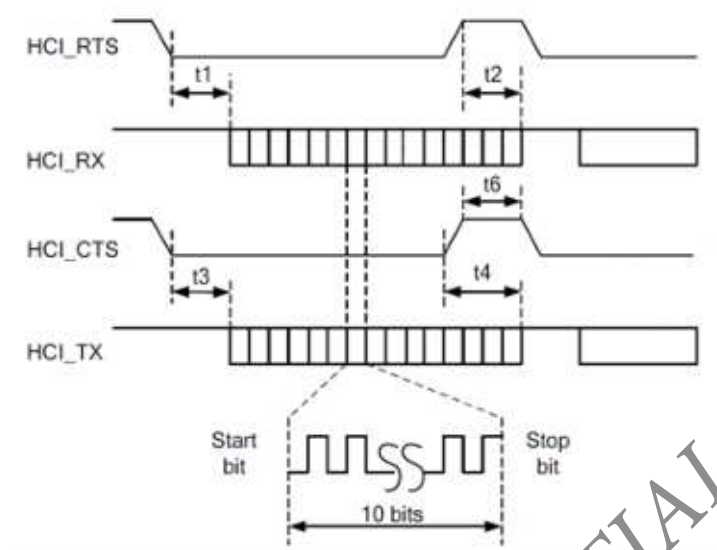
Figure 5-6. UART Timing Diagram
