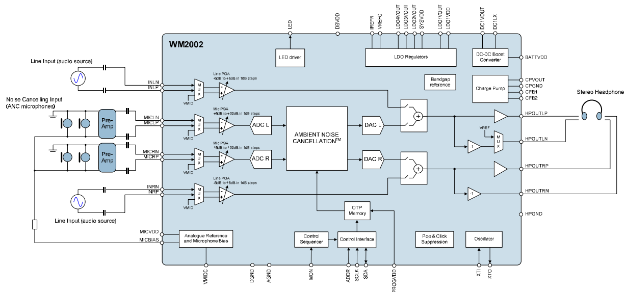
Figure 1 Typical Application
