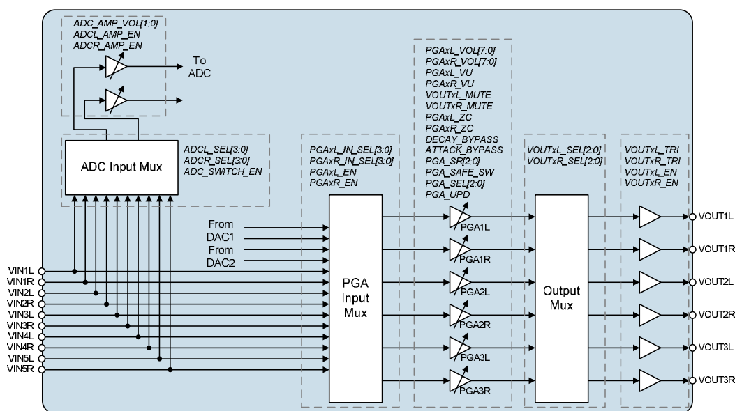
Figure 19 Analogue Routing Paths and Control
