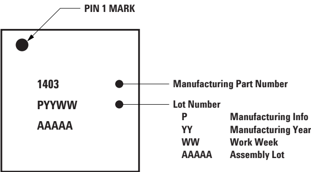
Figure 9. Marking specifications
