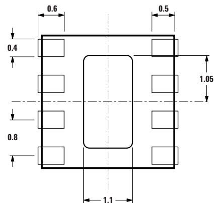
Figure 16. Solder paste stencil aperture
