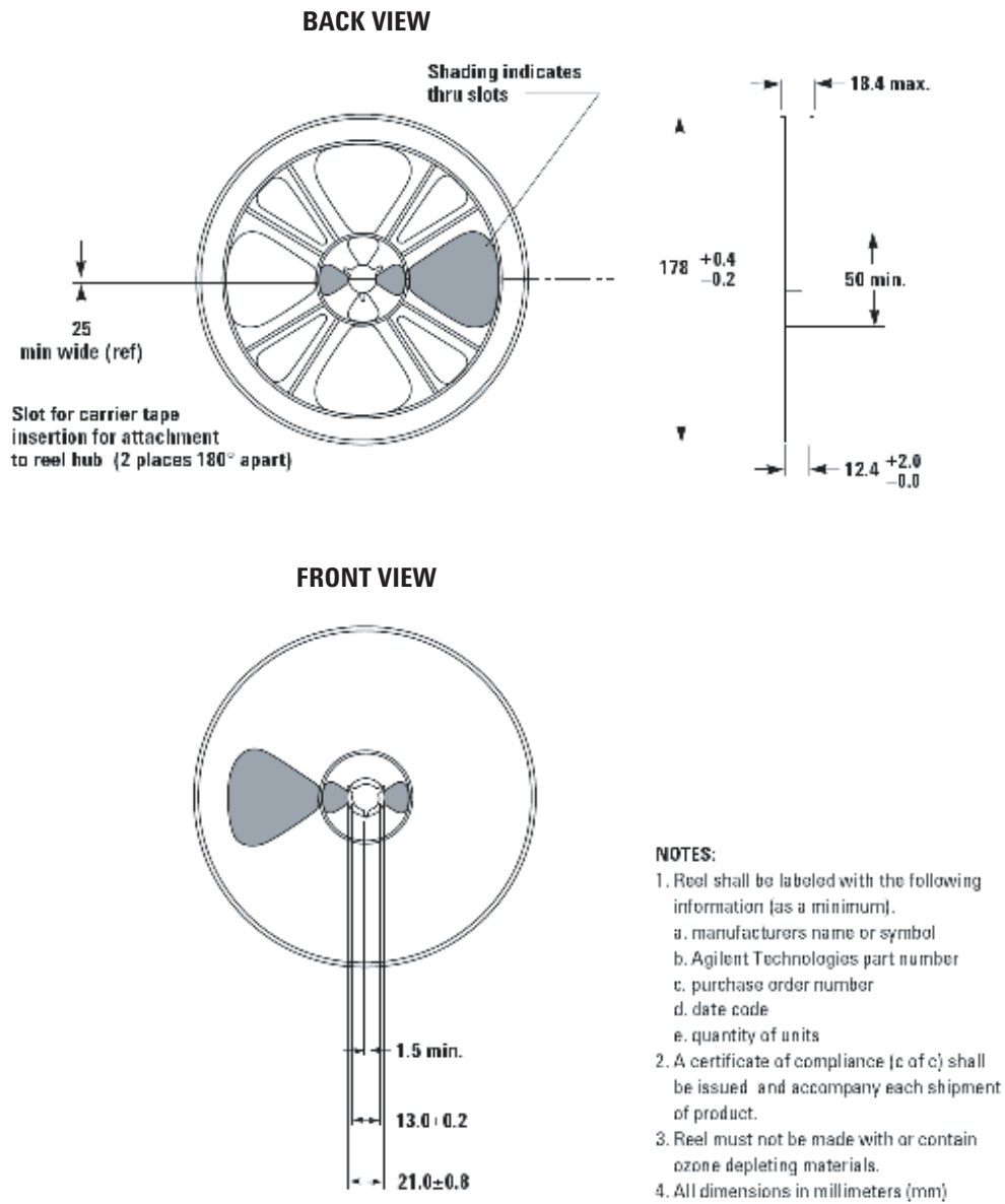
Figure 18. Plastic reel format (all dimensions are in millimeters)
