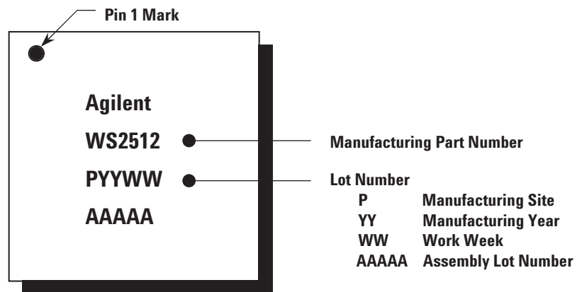
Figure 20. Marking Specification.
