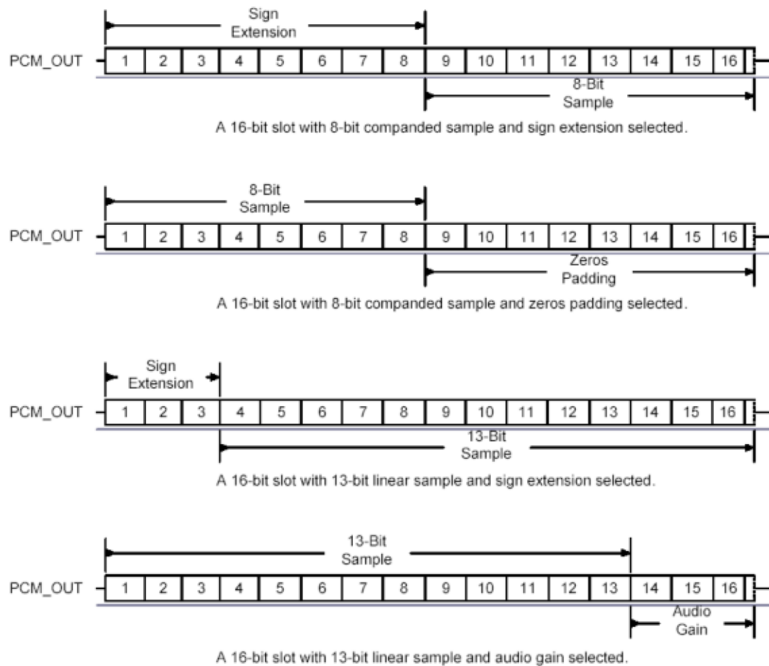
Figure 25: 16-bit Slot Length and Sample Formats
