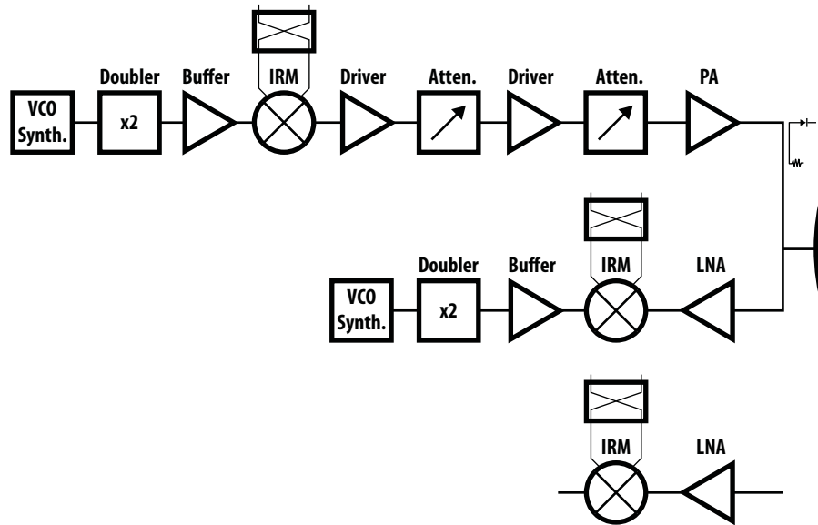
Microwave Link Packaged Suggested Solution 10-11 GHz
