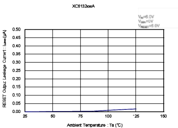
(13) RESET Output Leakage Current vs Ambient Temperature
