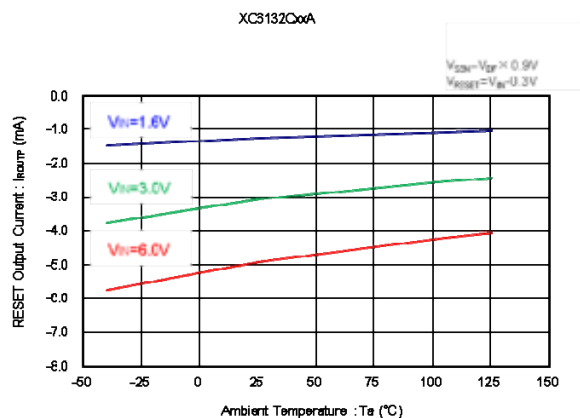
(11) RESET Output Current vs Ambient Temperature (Continued)
