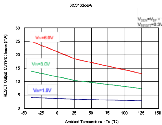
(11) RESET Output Current vs Ambient Temperature
