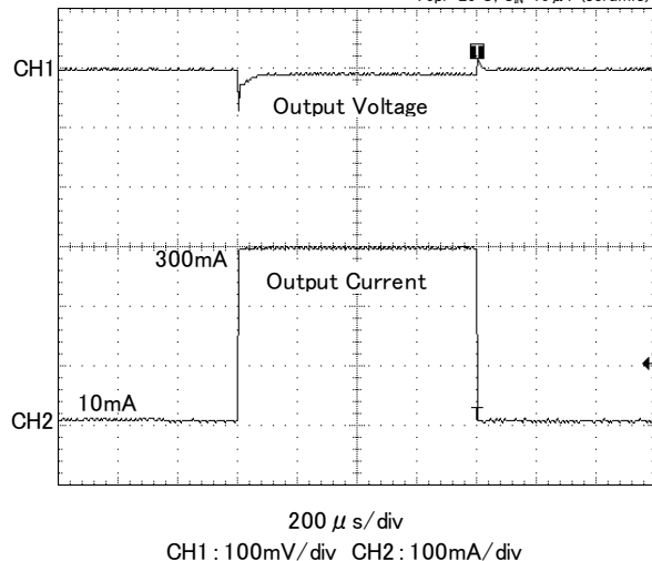
XC6220x501
