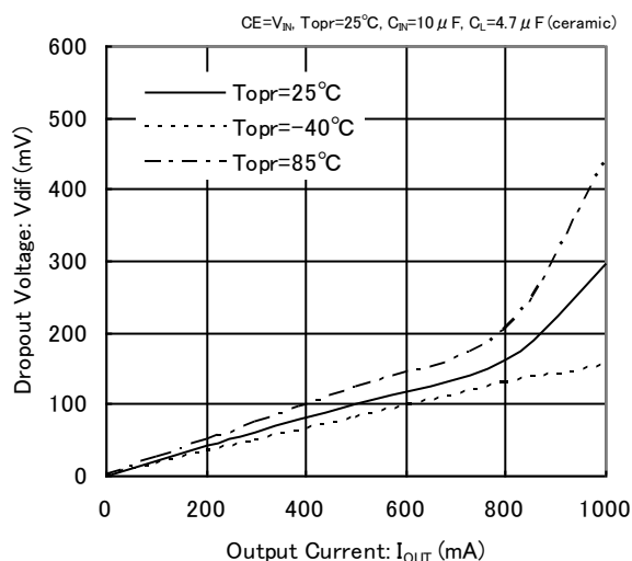
XC6220x301
