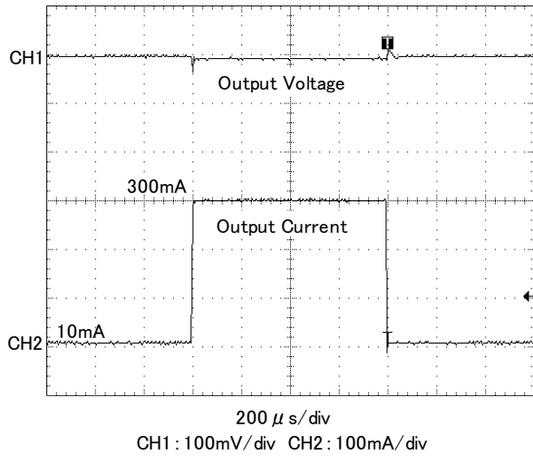
XC6220x301
