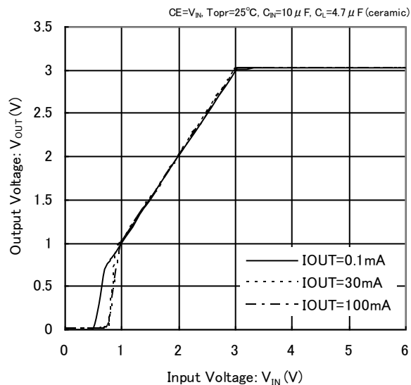
XC6220x301
