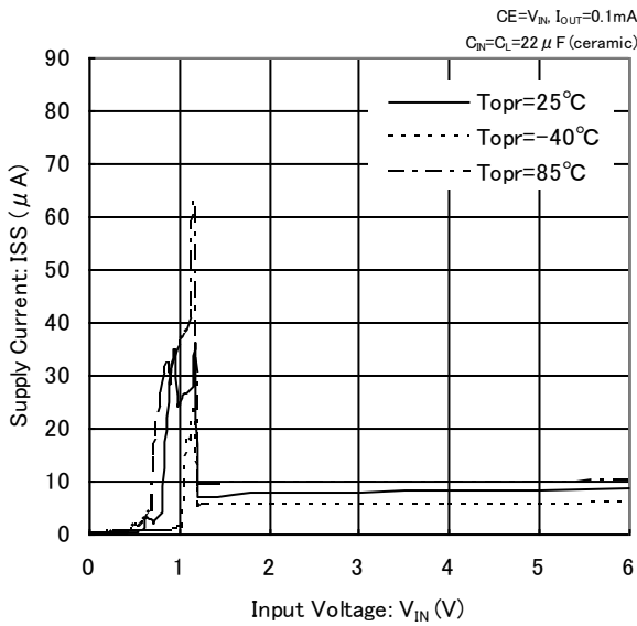
XC6220x121
