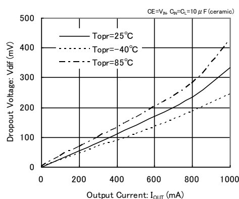
XC6220x181
