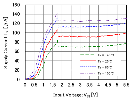
XC6223x181
