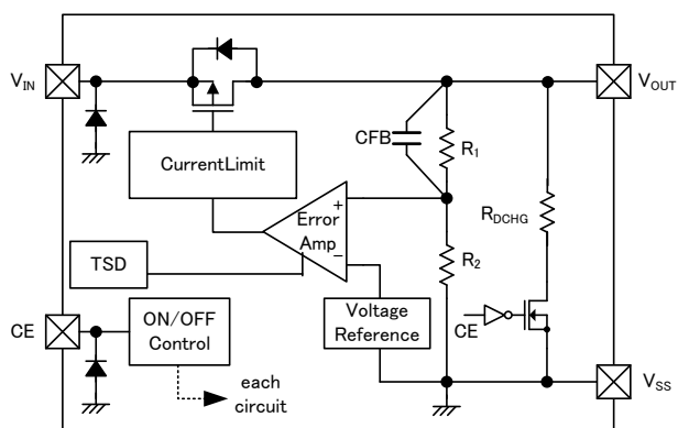
XC6223B/K
