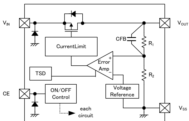
XC6223A/J
