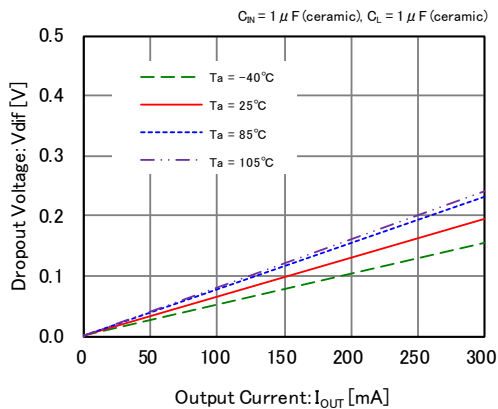
XC6223x251
