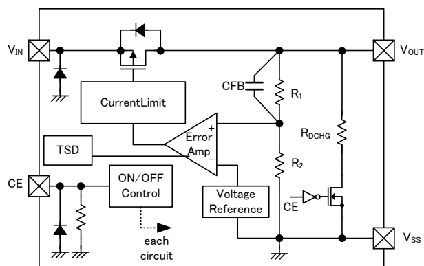
XC6223D/N
