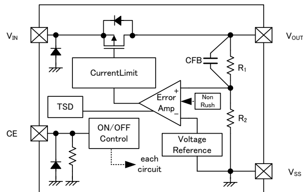
XC6223G/R
