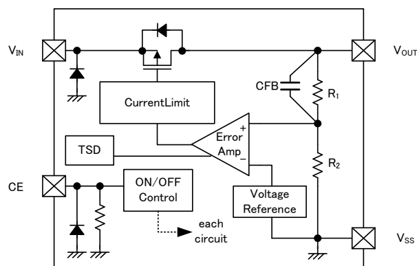
XC6223C/M
