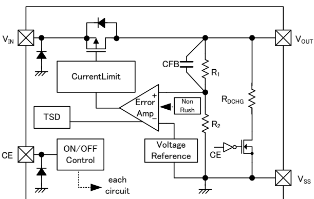
XC6223F/Q
