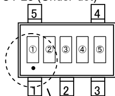
SOT-25 (Under-dot)
