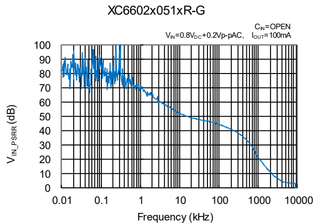
(17) Input Voltage Ripple Rejection
