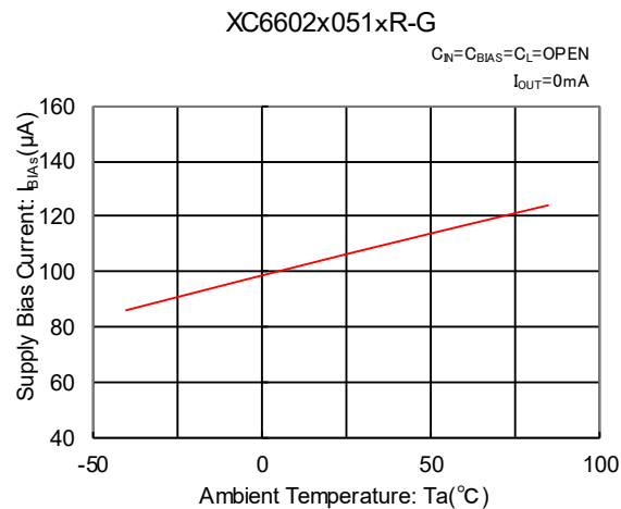
(8) Supply Bias Current vs. Ambient Temperature
