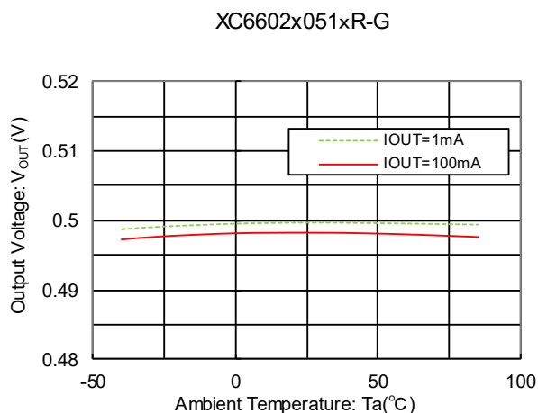
(7) Output Voltage vs. Ambient Temperature
