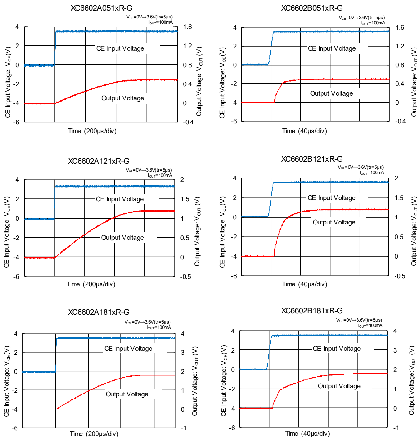
(14) CE Rising Response Time
