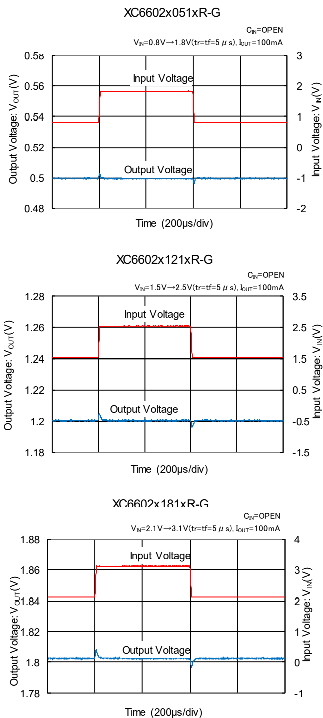
(11) Input Transient Response
