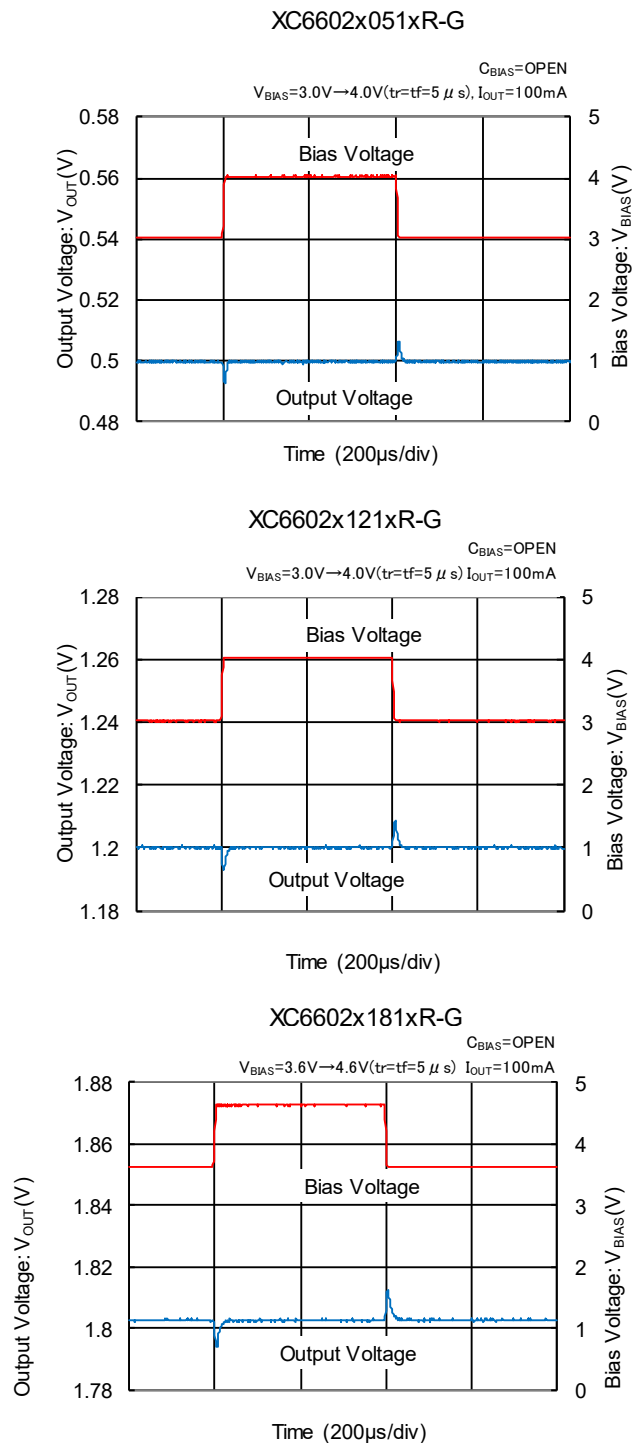
(10) Bias Transient Response
