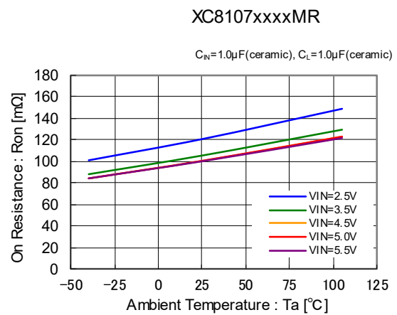
(10) On Resistance
