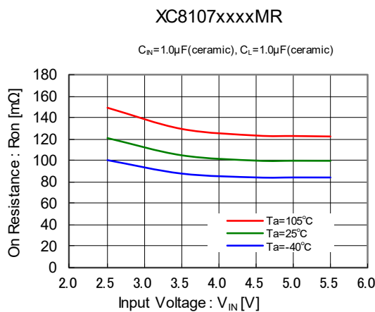
(9) On Resistance vs. Input Voltage (SOT-25:XC8107A,B)
