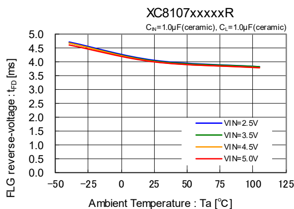
(18) FLG delay time reverse-voltage vs. Ambient Temperature
