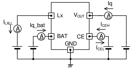
< Circuit No.④ >
