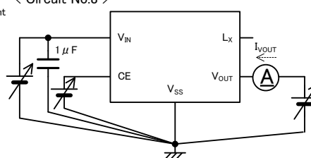
< Circuit No.8 >
