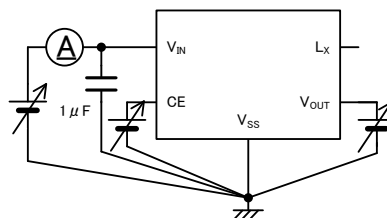
< Circuit No.2 >
