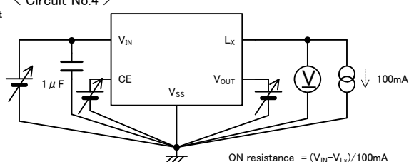
< Circuit No.4 >
