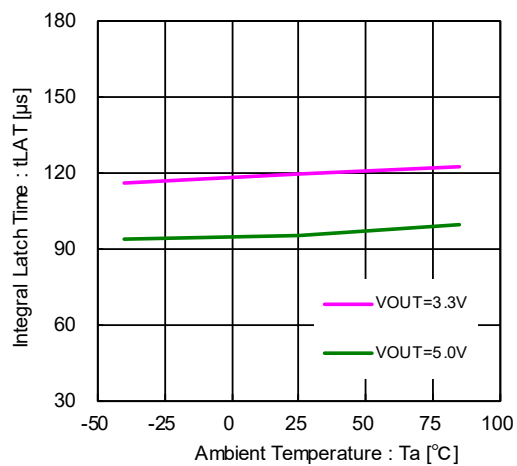
(23) Integral Latch Time vs. Ambient temperature
