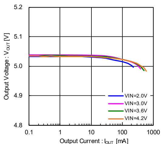
XCL102D503CR-G/XCL102E503CR-G
