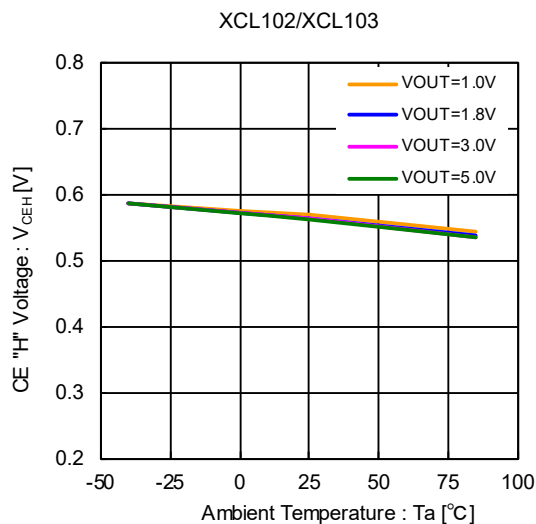
(12) CE "H" Voltage vs. Ambient Temperature
