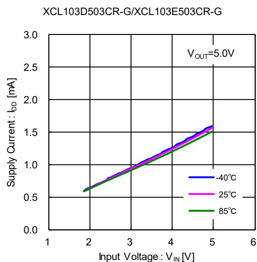
(6) Supply Current vs. Input Voltage
