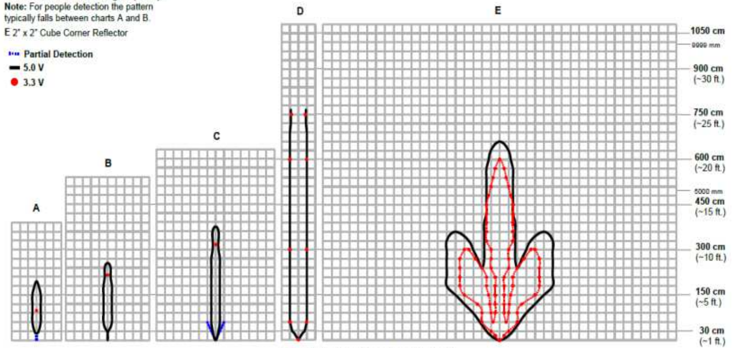
Beam Characteristics are Approximate Beam Pattern drawn to a 1:95 scale for easy comparison to our other products.
