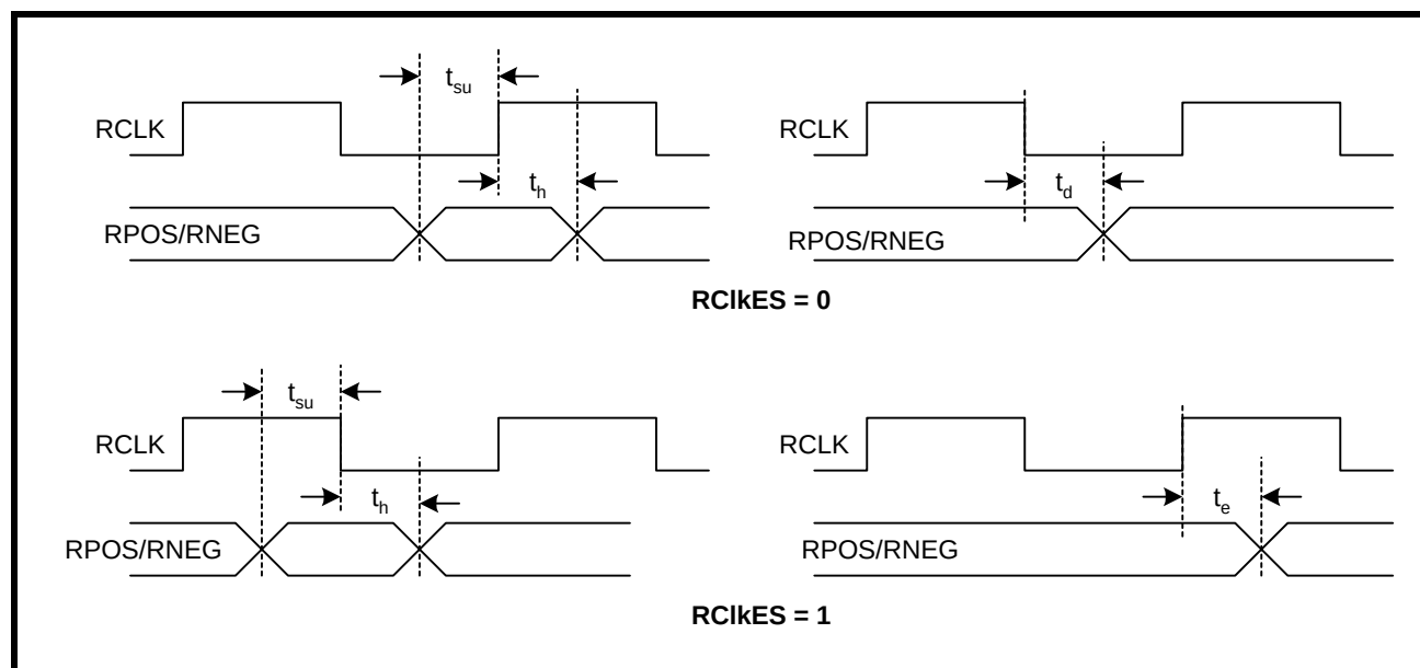
FIGURE 3. INPUT/OUTPUT TIMING
